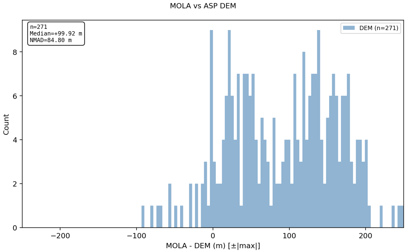
Figure 7: Distribution of elevation differences between MOLA and ASP DEM.
