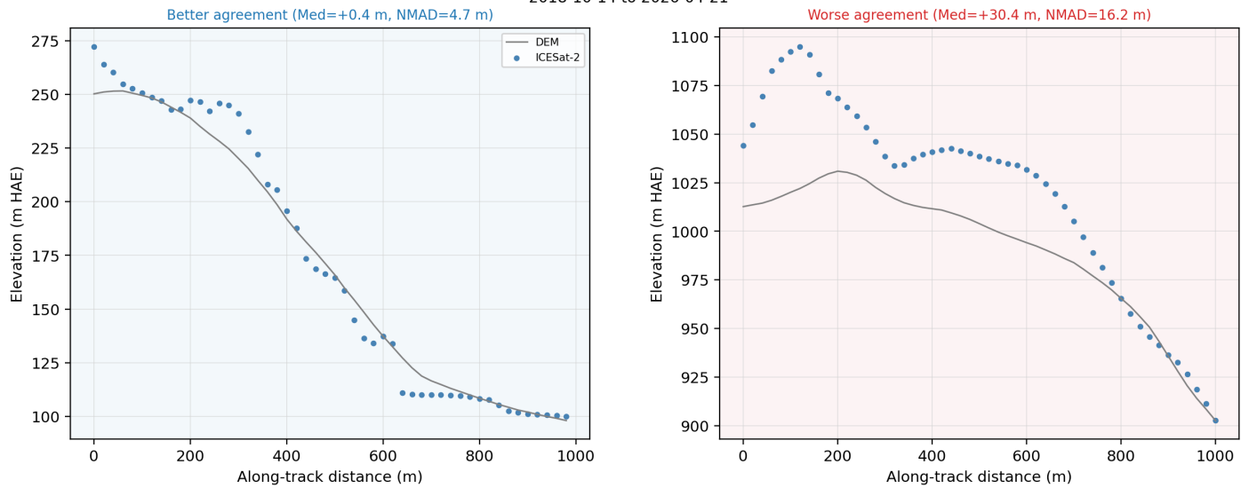
Figure 9: 1 km segments along the ICESat-2 track with better (left) and worse (right) agreement with the DEM. Segments are scored by 3 \cdot |\text{median}(dh)| + \text{NMAD}(dh) , which weights the median bias three times more than the dispersion so that a segment with a large bias is not selected as 'better agreement' just because its NMAD is small.
