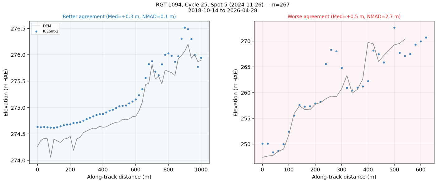
Figure 12: 1 km segments along the ICESat-2 track with better (left) and worse (right) agreement with the DEM. Segments are scored by 3 \cdot |\text{median}(dh)| + \text{NMAD}(dh) , which weights the median bias three times more than the dispersion so that a segment with a large bias is not selected as 'better agreement' just because its NMAD is small.
