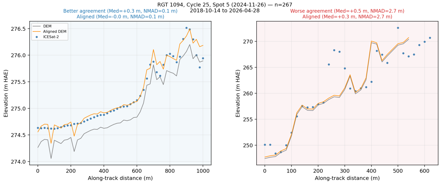
Figure 16: The same better- and worse-agreement segments as above, now with the aligned DEM overlaid. Segment selection is held fixed so Median/NMAD can be compared directly.
