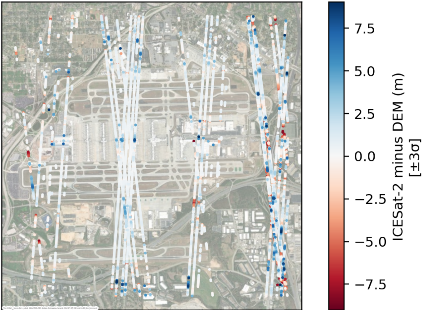
Figure 9: ICESat-2 ATL06-SR elevation differences vs. ASP DEM.
