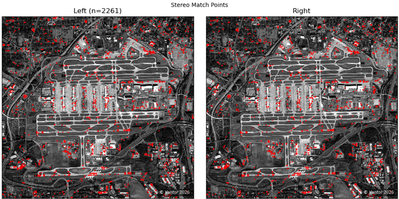
Figure 3: Interest point matches between left and right images. These are produced by stereo_corr during its initial interest point matching step, which is used to set the search windows for subsequent dense correlation (not the dense correlation matches themselves).
